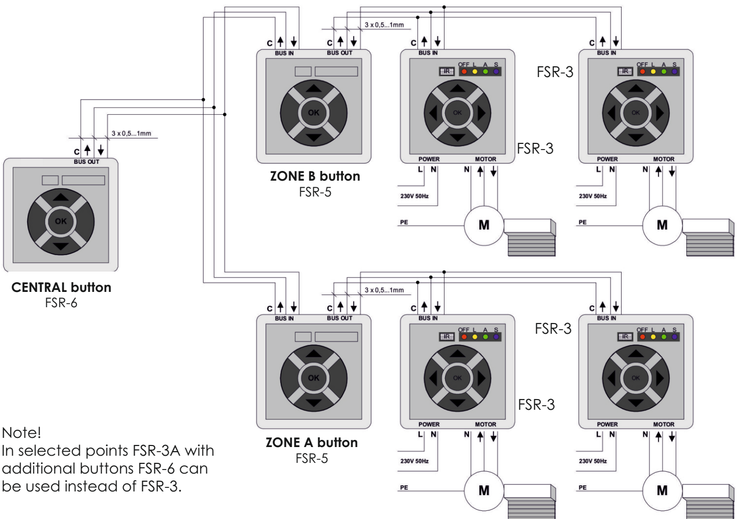
Diagram no. 4 System with division into two zones A and B (2 x FSR-5 + 2 x (n x FSR-3)) version with additional central button FSR-6
