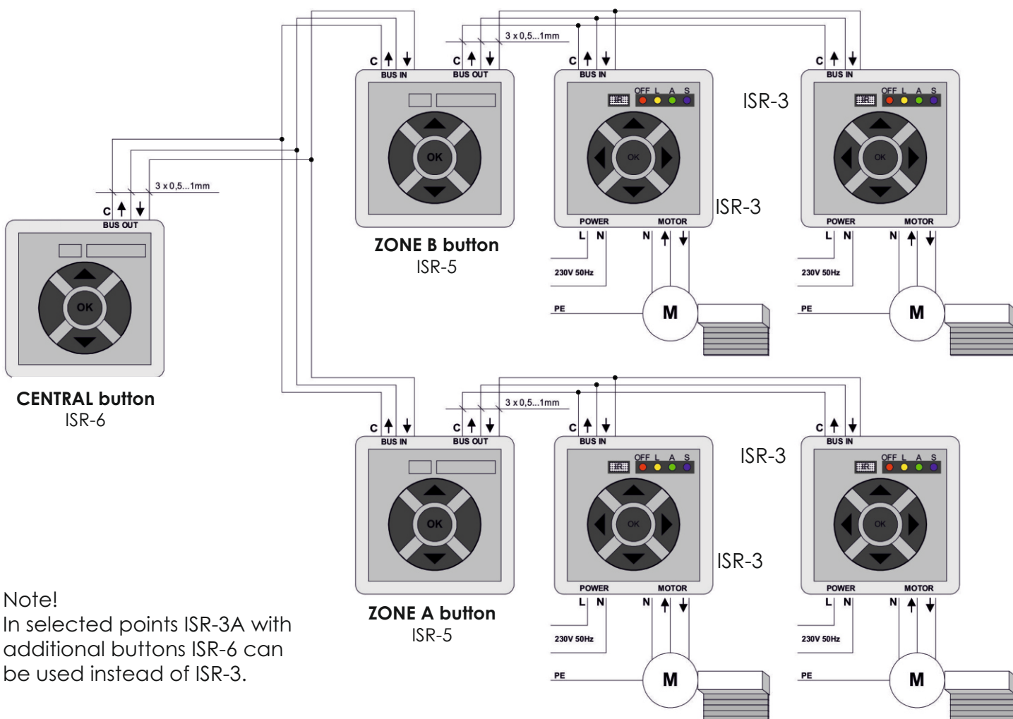
Diagram no. 4 System with division into two zones A and B (2 x ISR-5 + 2 x (n x ISR-3)) version with additional
