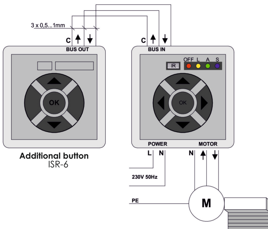
Diagram no. 2 ISR-3 version with additional button ISR-6
